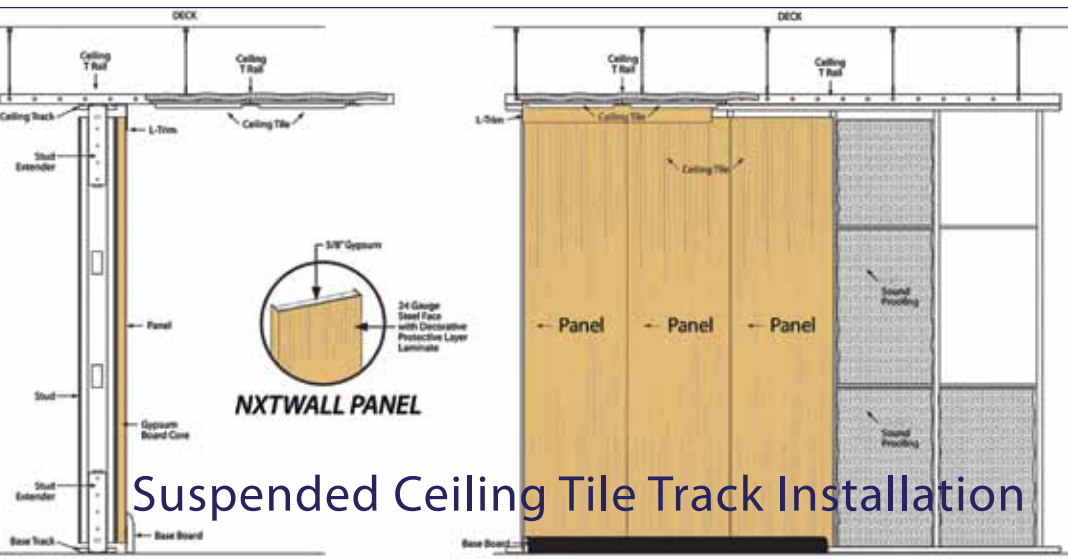
CEILING INTERFACE
